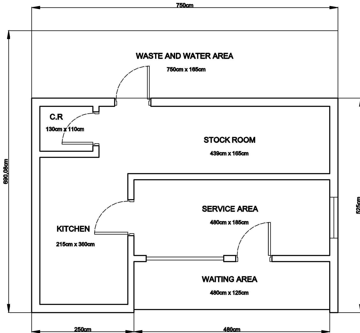
2D FLOOR PLAN
